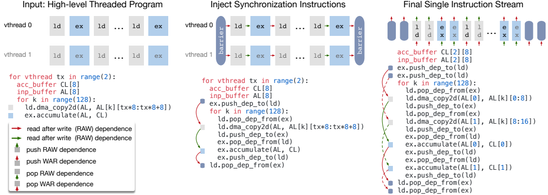
Figure 8: TVM virtual thread lowering transforms a virtual thread-parallel program to a single instruction stream; the stream contains explicit low-level synchronizations that the hardware can interpret to recover the pipeline parallelism required to hide memory access latency.
